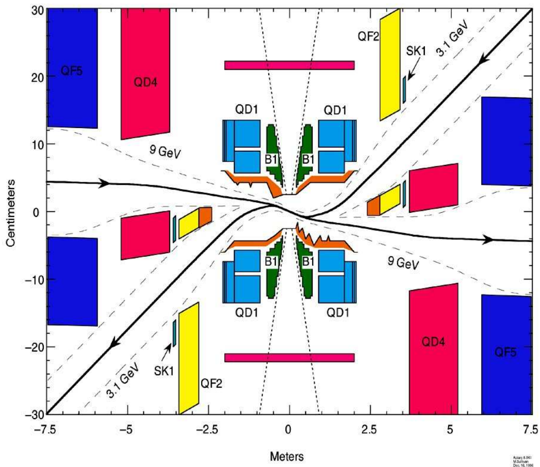
Figure 3.2: The Interaction Region
