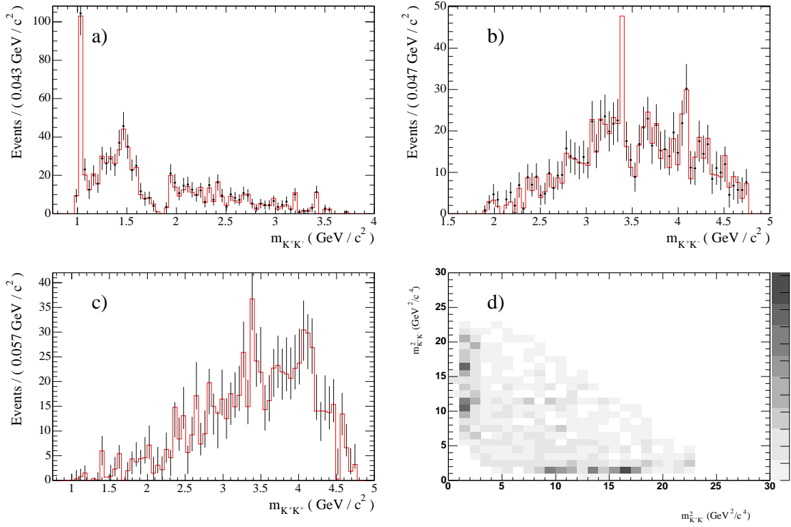
Figure 5.12: Background subtracted (red histogram) and s Plot (black points) comparison for B^+ data. Sub-figure a) shows the K^+K^- mass spectrum for the lower mass combination, b) shows the K^+K^- higher mass combination, and c) shows the K^+K^+ spectrum. The s Plot Dalitz plot distribution is shown in d).
