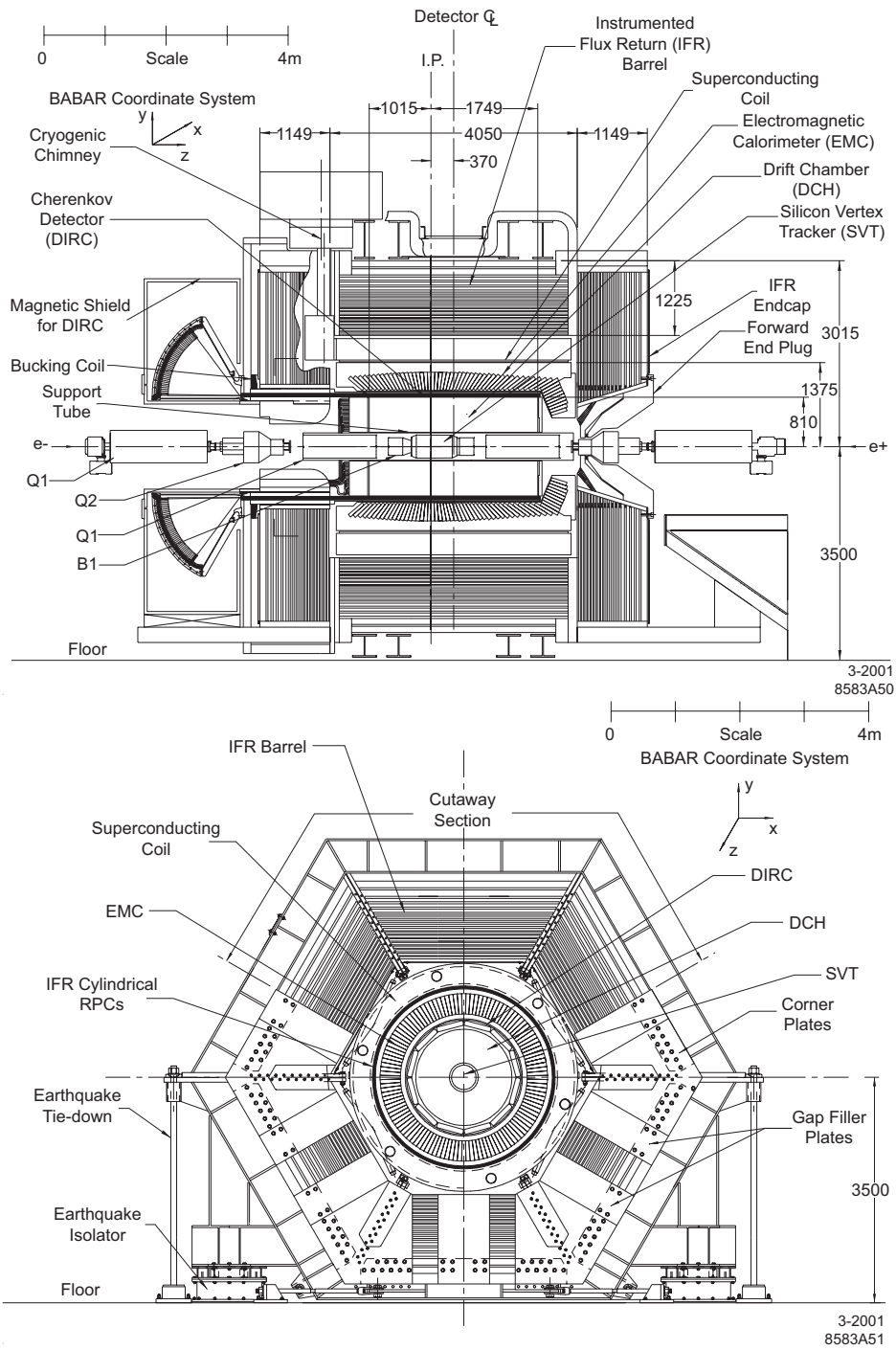
Figure 3.4: The BABAR detector [46].
