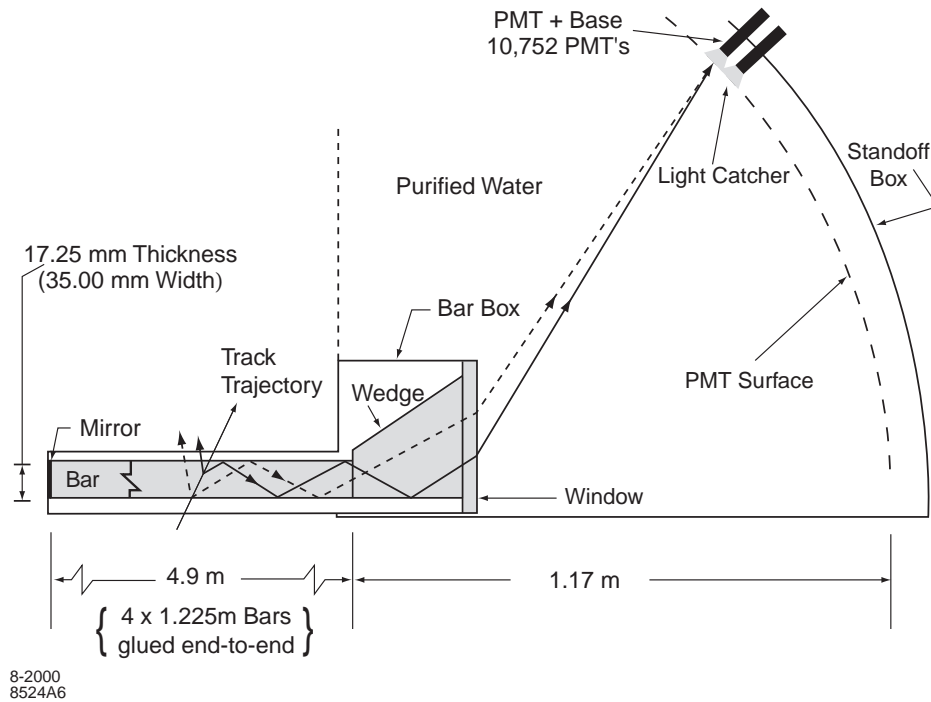
Figure 3.13: Diagram showing DIRC principles of operation [46].
