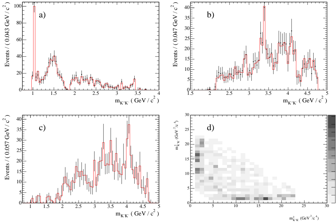
Figure 5.13: Background subtracted (red histogram) and s Plot (black points) comparison for B^- data. Sub-figure a) shows the K^+K^- mass spectrum for the lower mass combination, b) shows the K^+K^- higher mass combination, and c) shows the K^-K^- spectrum. The s Plot Dalitz plot distribution is shown in d).
