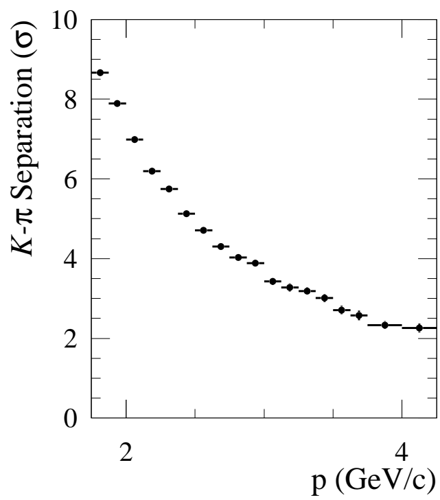
Figure 3.14: Kaon-Pion separation with the DIRC, as a function of momentum.
