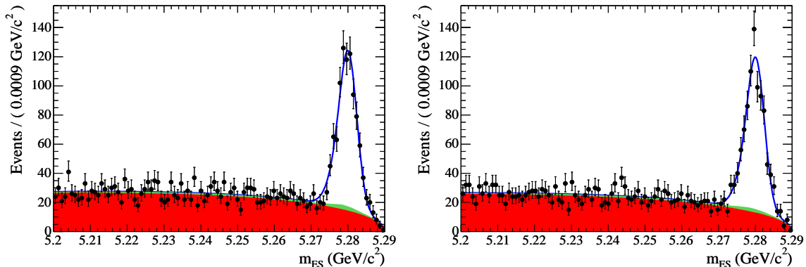
Figure 5.4: The projection in m_{ES} for signal strip events. The data are shown as solid points, the fit is shown as a blue line, and the solid red and green areas show the continuum and B -related backgrounds respectively. The two charge samples are shown separately: left hand subfigure — the B^+ sample; right hand subfigure — the B^- sample.
