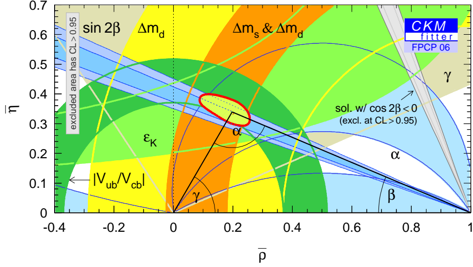
Figure 2.4: Constraints on The Unitarity Triangle, focusing on the \alpha vertex in the \bar{\rho} - \bar{\eta} plane [17].
