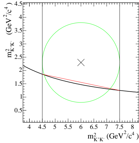
Figure 5.22: The Dalitz plot boundary (curved black line) can be approximated as a straight line (solid red line), by calculating the boundary value at the edges of the volume (green circle with edges shown as two vertical black lines), and joining these points.
